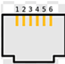
RS232 RJ12 Socket Pinout
