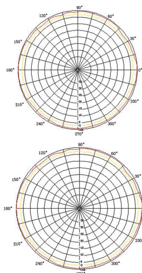
Vertical Pattern (698-960/1710-2170)
